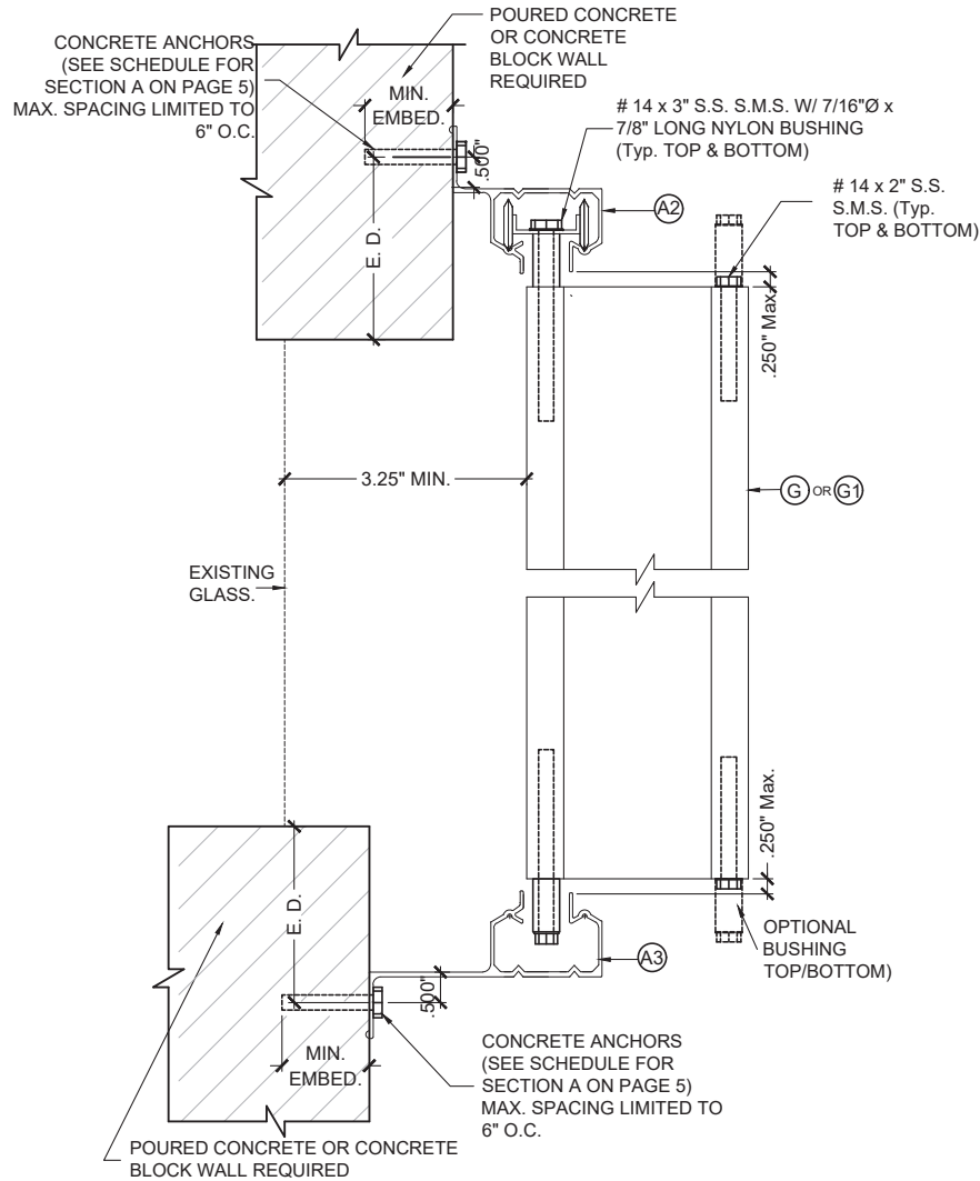
SECTION L1 SCALE : 3/8" = 1"
