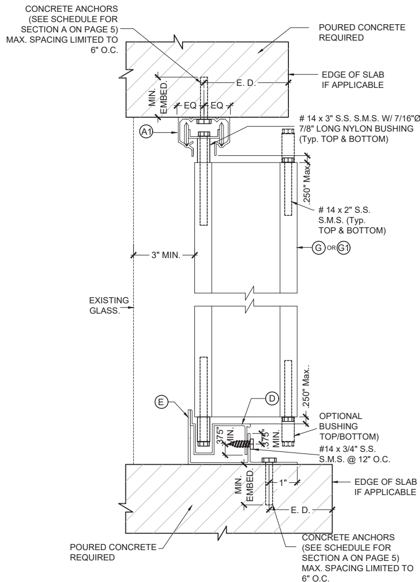
SECTION L2 SCALE : 3/8" = 1"
