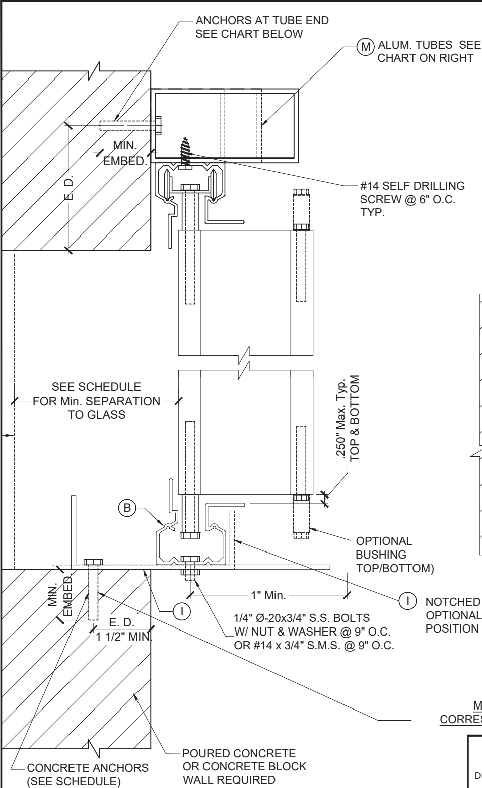
BUILD-OUT INSTALLATION SECTION M
